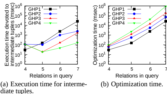
Figure 9: Varying the number of relations and GHP iterations.
