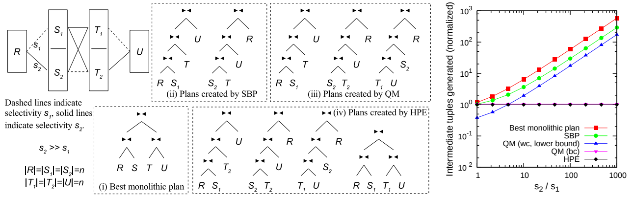
(a) Running example query and the join plans chosen by a (i) a traditional query optimizer, (ii) selectivity-based partitioning [18], (iii) query mesh [17], and (iv) our approach. (b) Intermediate tuples generated (normalized).
