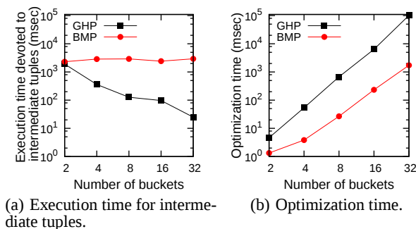
Figure 8: The effect of the number of histogram buckets.
